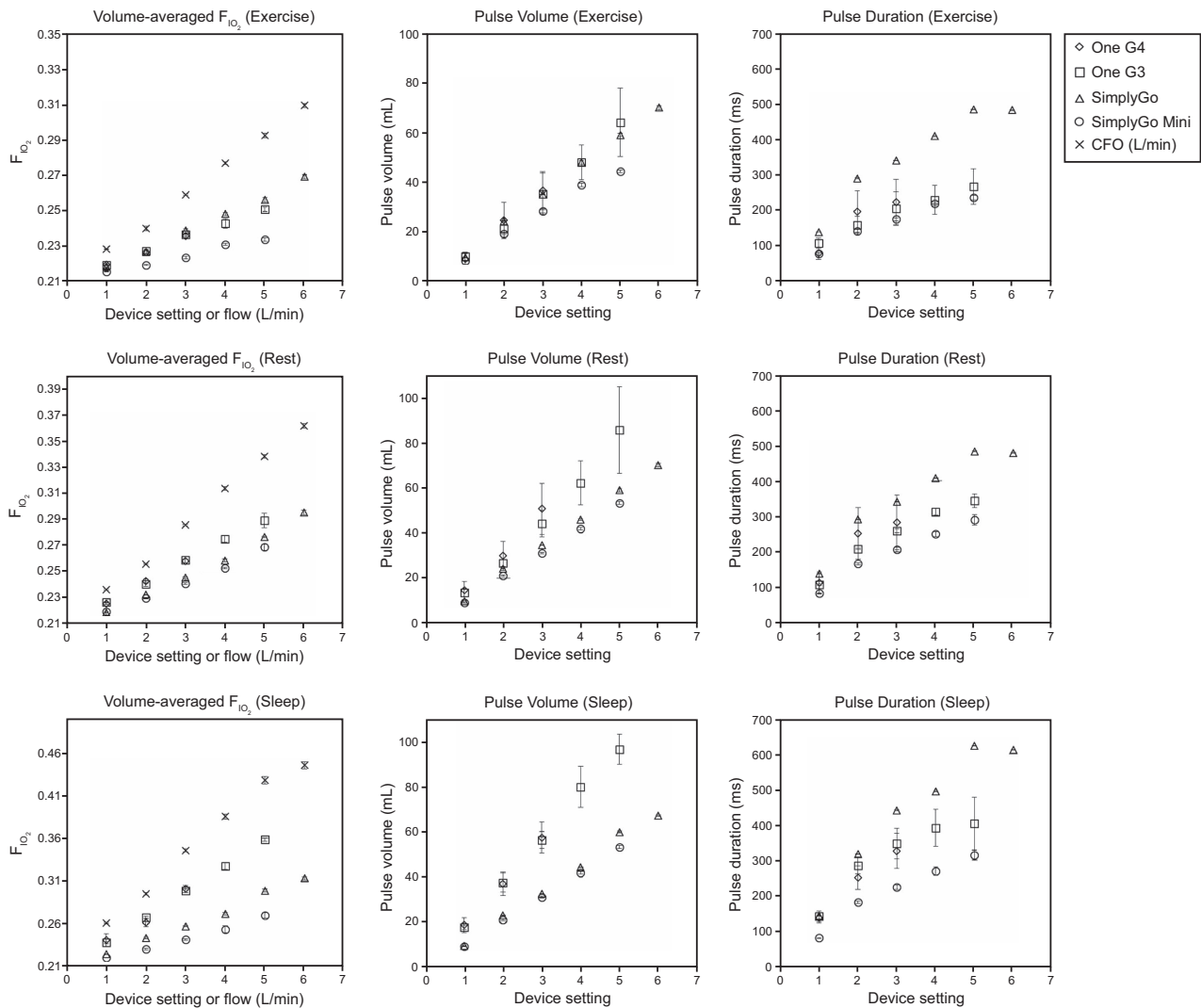
Fig. 5. Volume-averaged F_{IO_2} and pulse characteristics for each of the tested portable oxygen concentrators and continuous flow oxygen across 3 breathing patterns. F_{IO_2} values were averaged over 5 consecutive breaths. Other pulse characteristics averaged >20 consecutive breaths. Error bars indicate \pm 1 SD.
